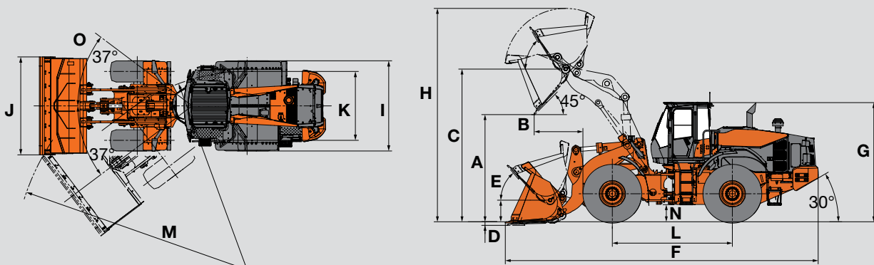
Equipped with 26.5R25 (L3) tire and ROPS cab.
