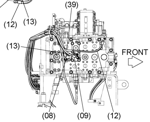
矢視 C VIEW C
