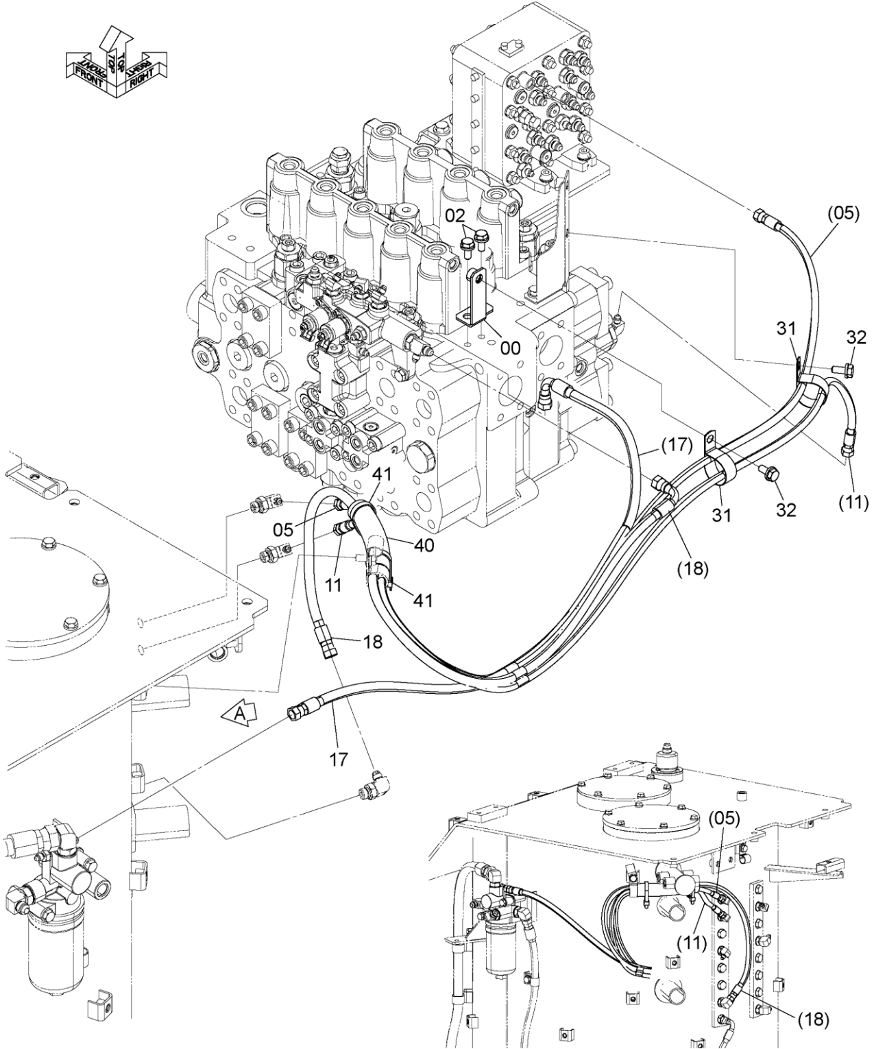
矢視 A VIEW A
