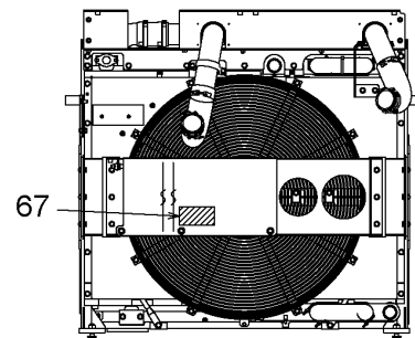
矢示 VIEW E
